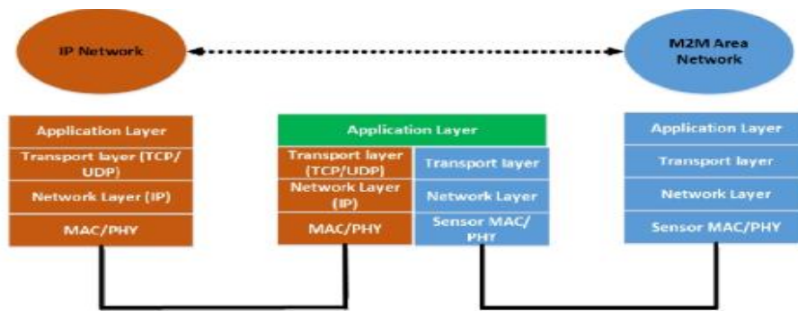
Fig. : Non-IP based M2M Network
